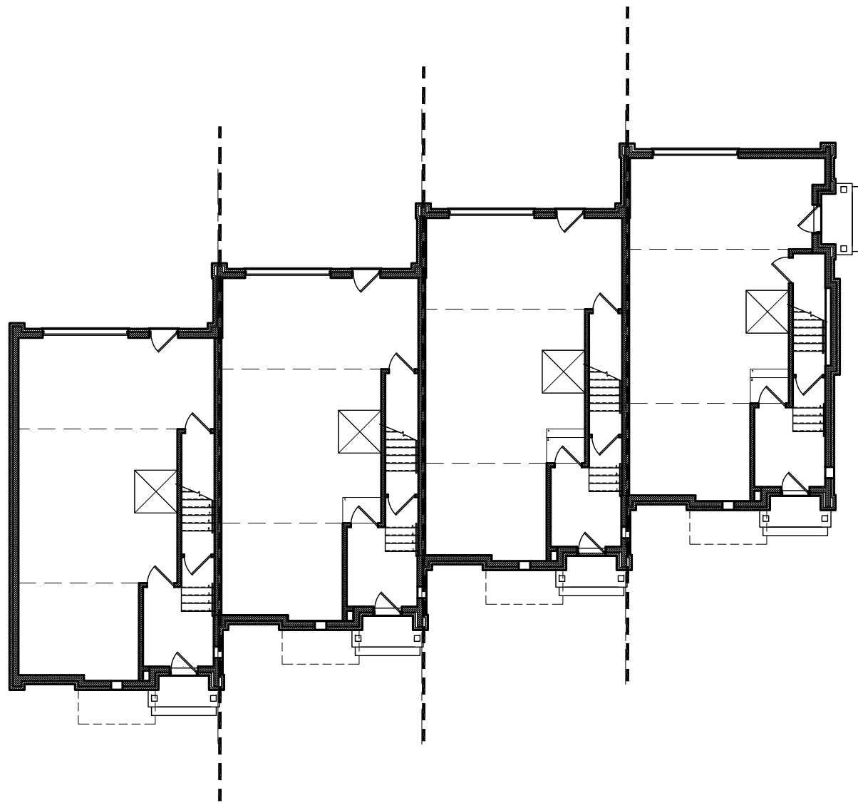
2 G-101 FIRE RATED WALL Scale: 1/16" = 1'-0"
