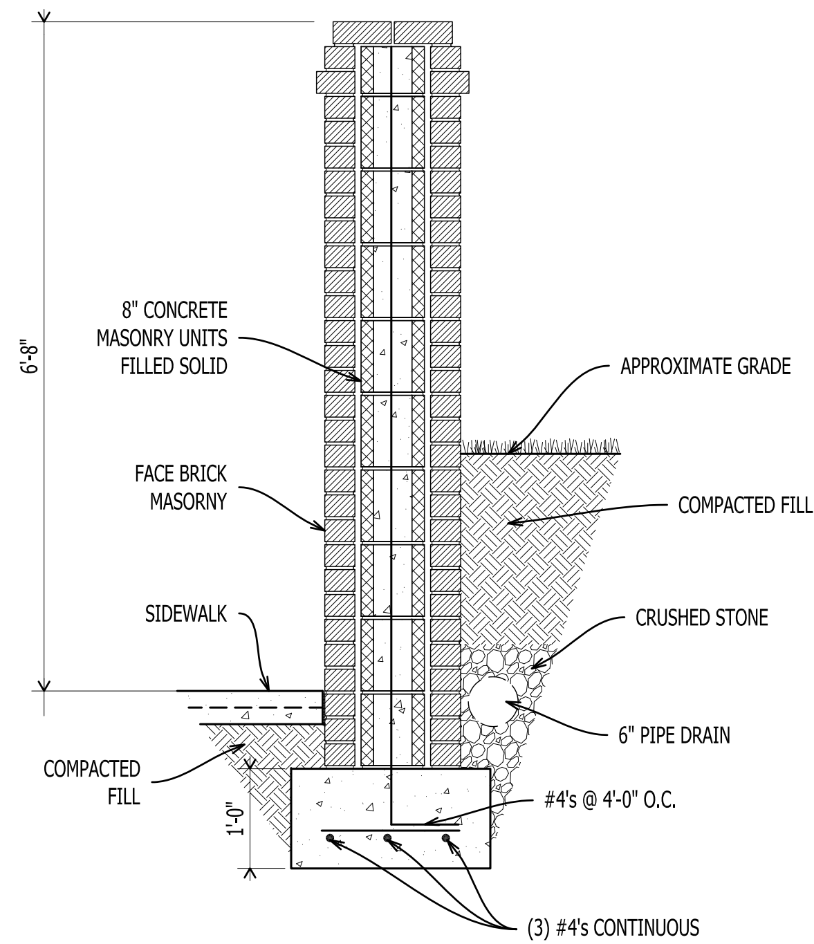
1 A-503 WALL DETAIL Scale: 3/4" = 1'-0"
