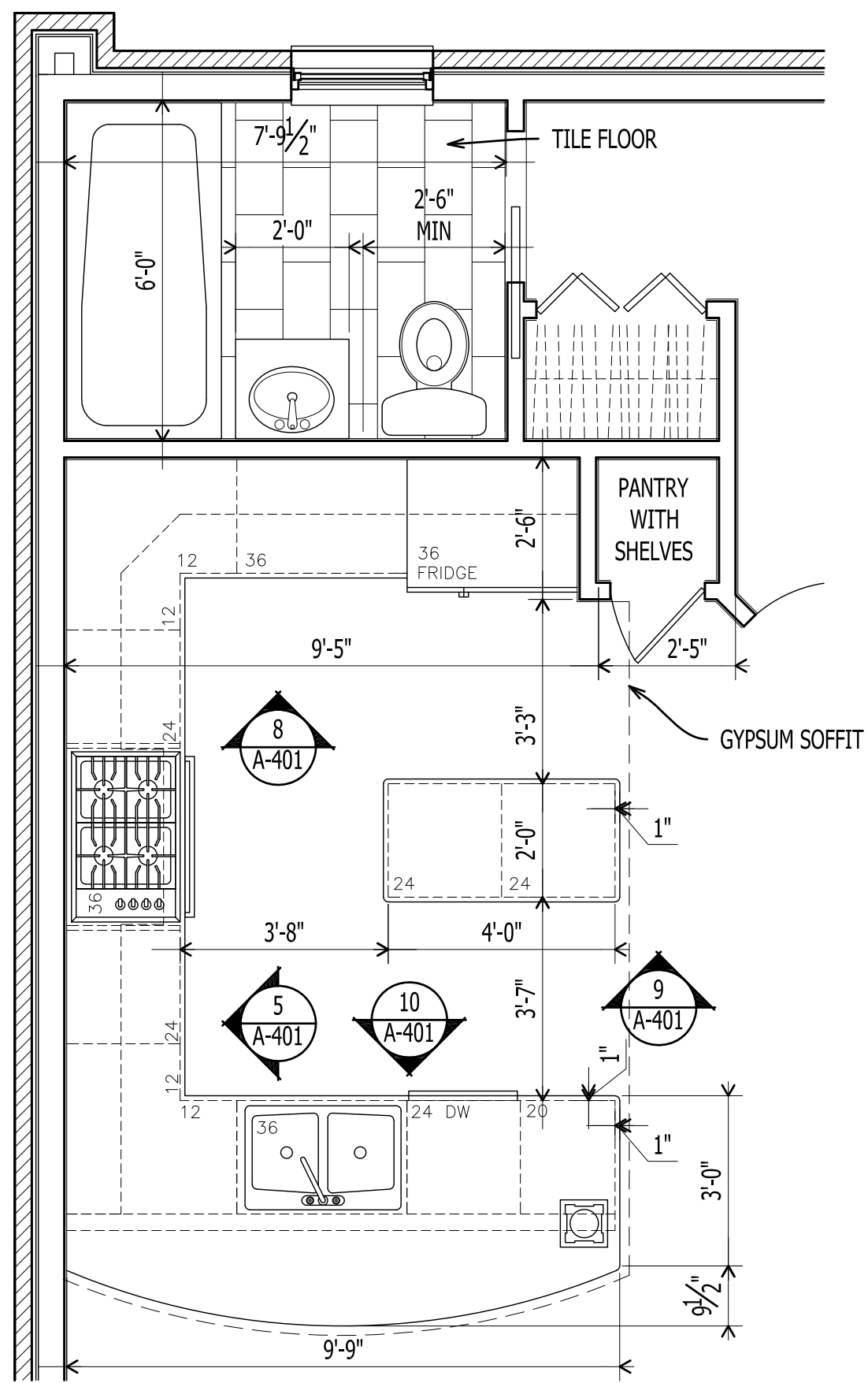
1 A-401 ENLARGED KITCHEN PLAN Scale: 3/8" = 1'-0"
