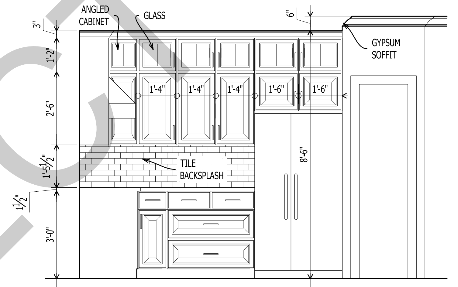
8 A-401 KITCHEN ELEVATION Scale: 1/2" = 1'-0"
