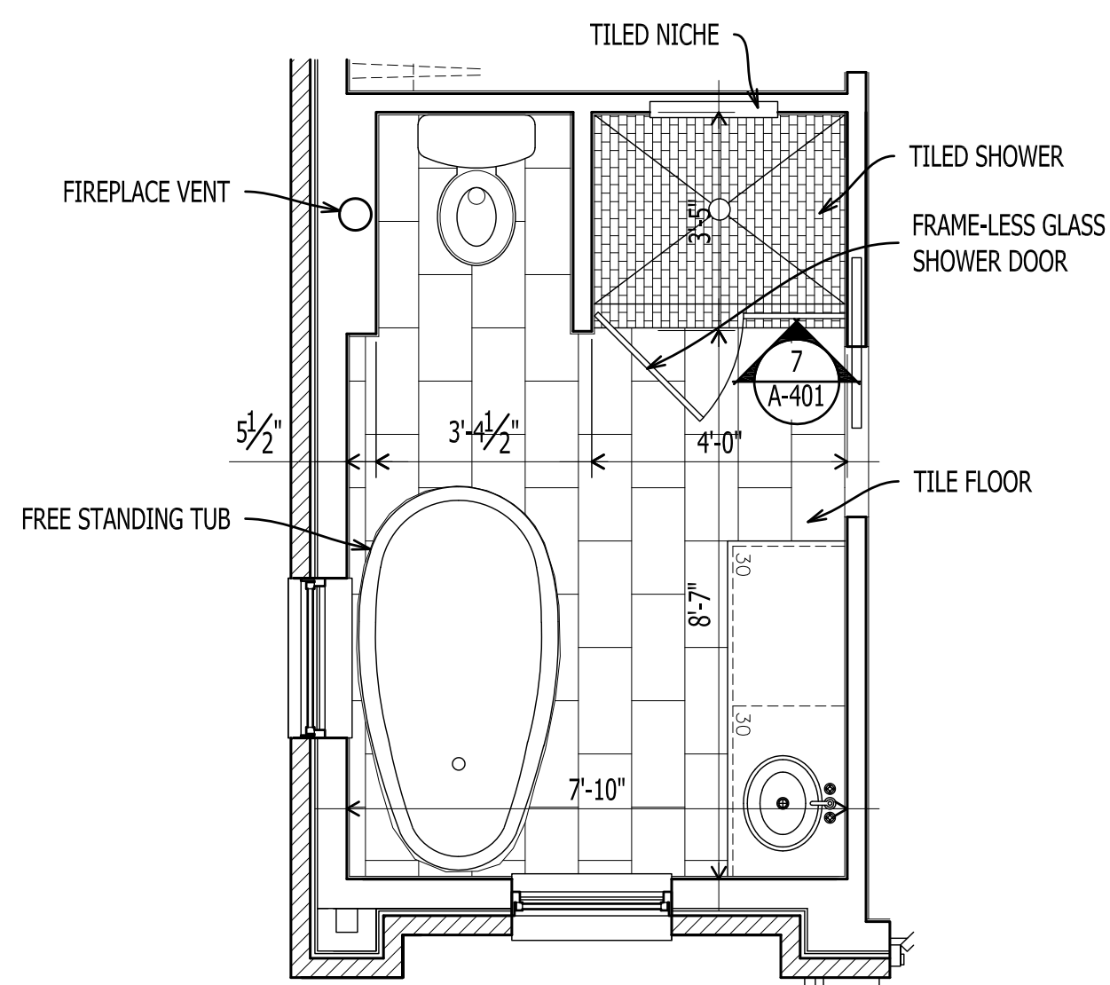
2 A-401 ENLARGED BATHROOM PLAN Scale: 3/8" = 1'-0"
