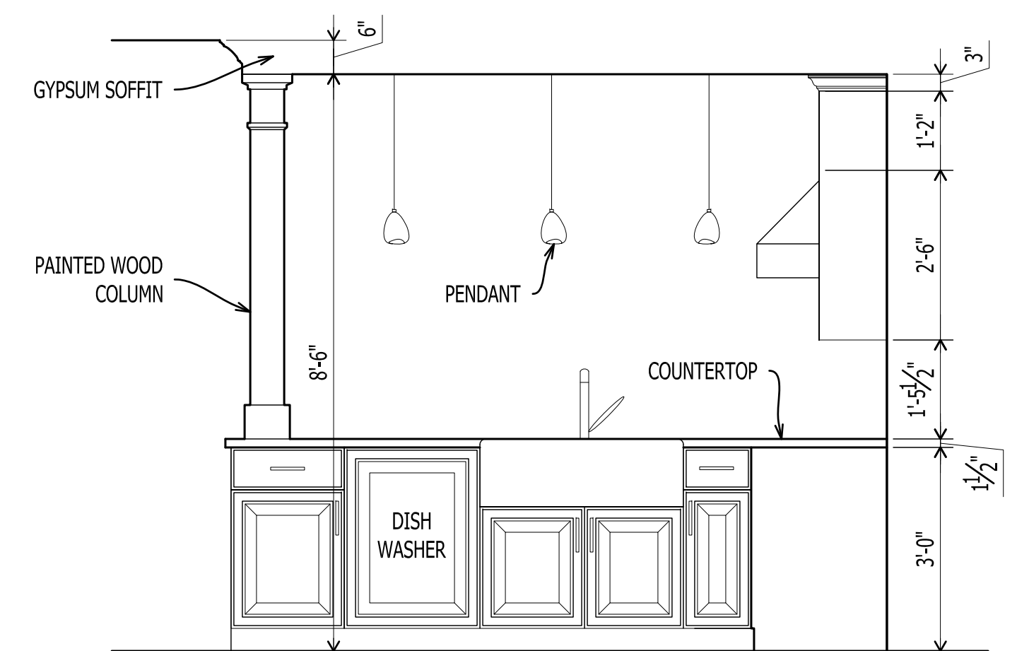
10 A-401 KITCHEN ELEVATION Scale: 1/2" = 1'-0"
