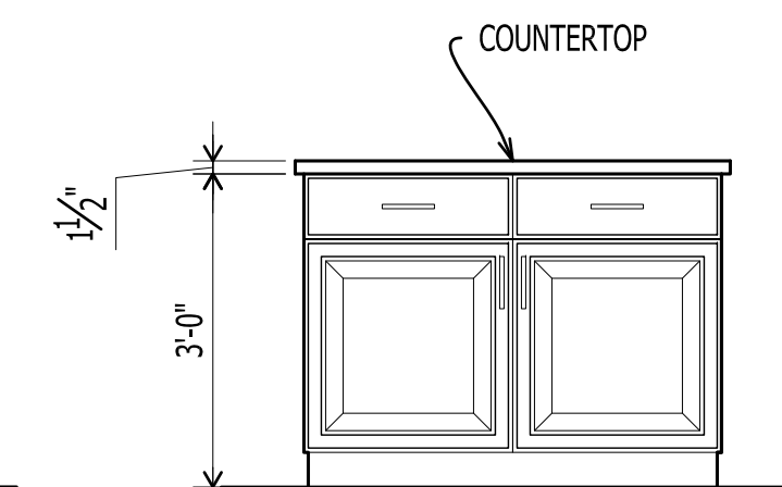
9 A-401 KITCHEN ELEVATION Scale: 1/2" = 1'-0"
