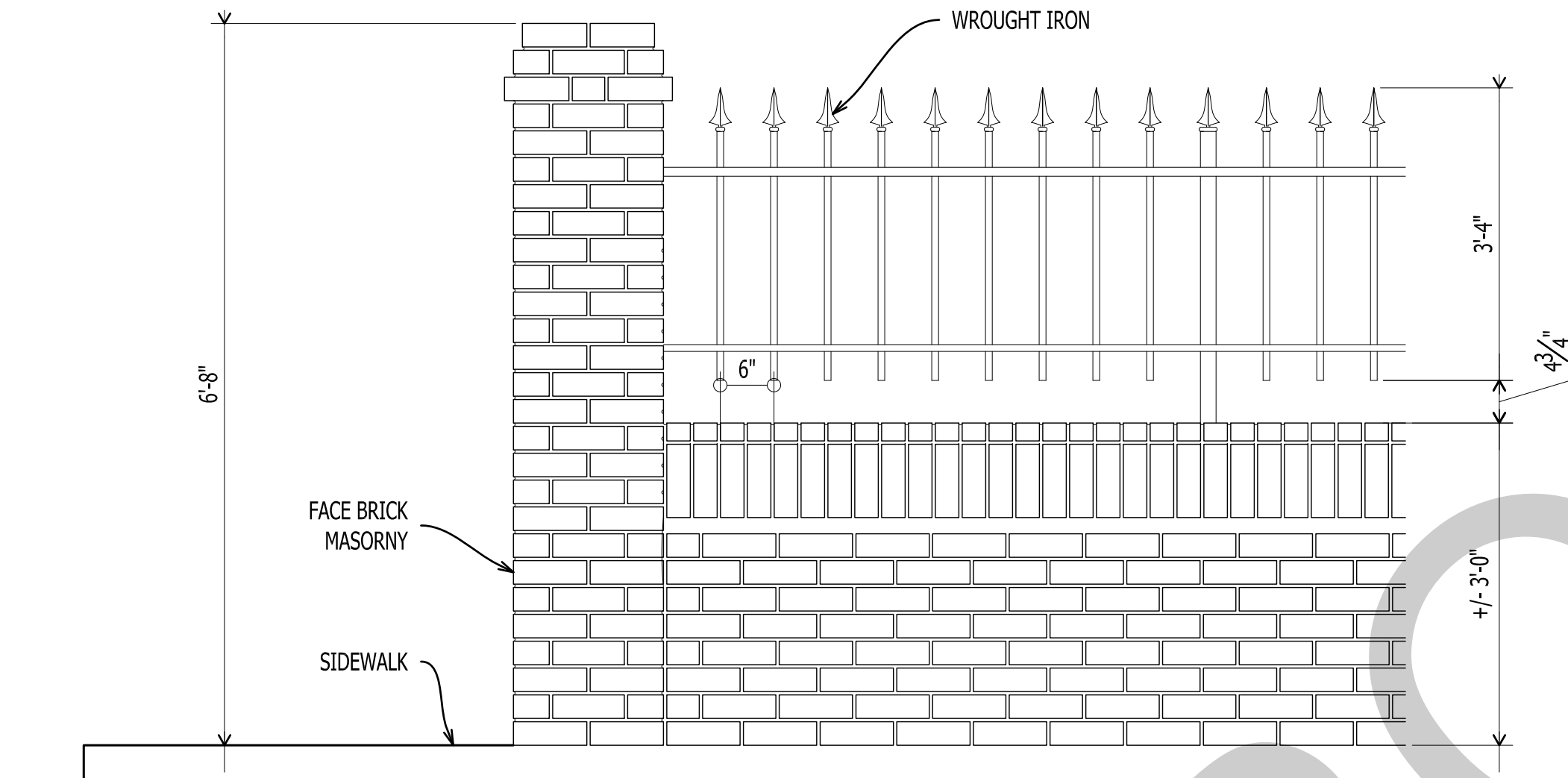
2 A-503 WALL DETAIL Scale: 3/4" = 1'-0"
