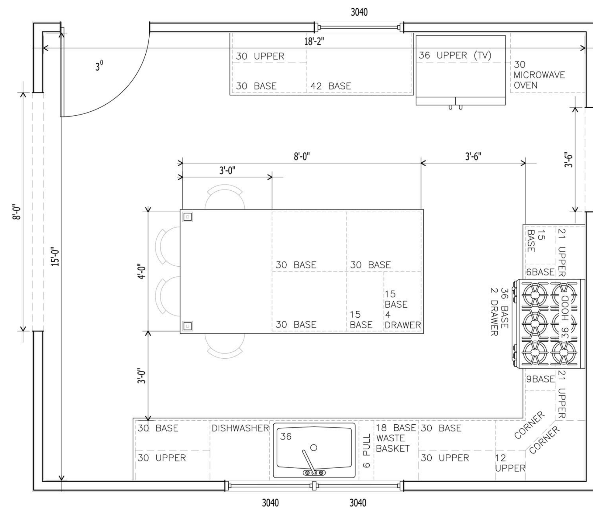
1 KITCHEN PLAN Scale: 1/2 = 1'-0"
