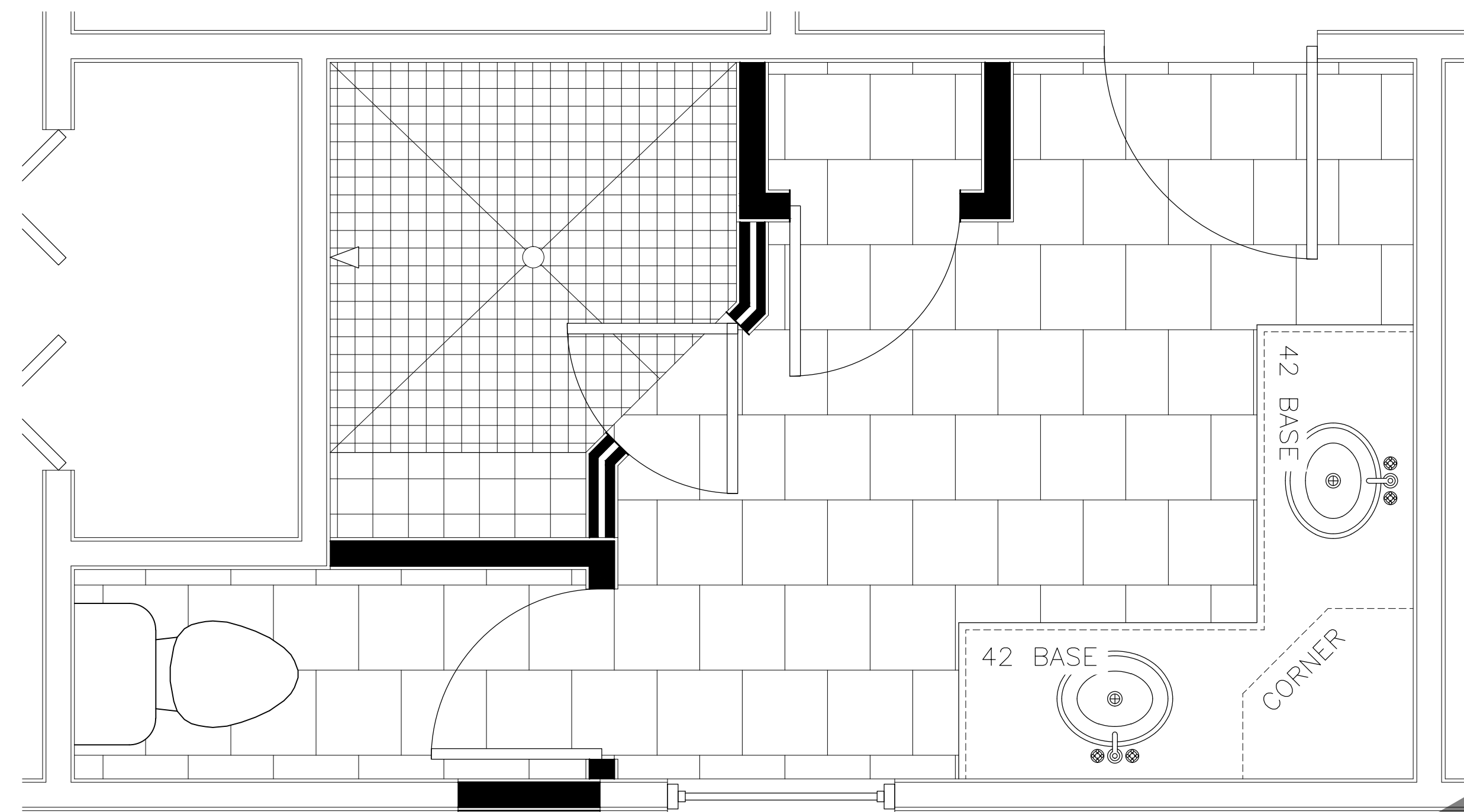
1 MASTER BATHROOM ENLARGED PLAN A-301 Scale: 3/4" = 1'-0"
