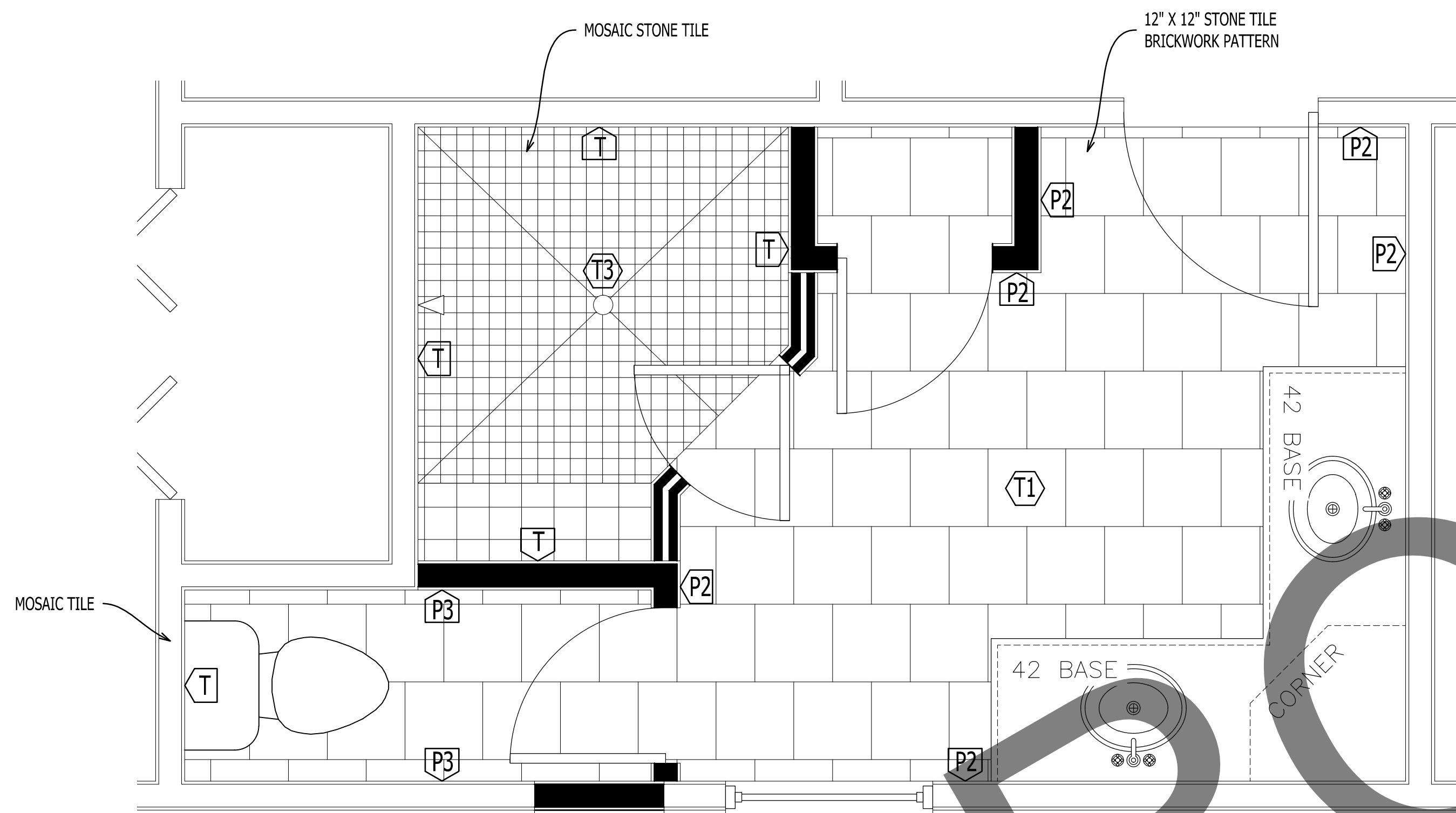
1 A-301 MASTER BATHROOM ENLARGED PLAN Scale: 3/4" = 1'-0"
