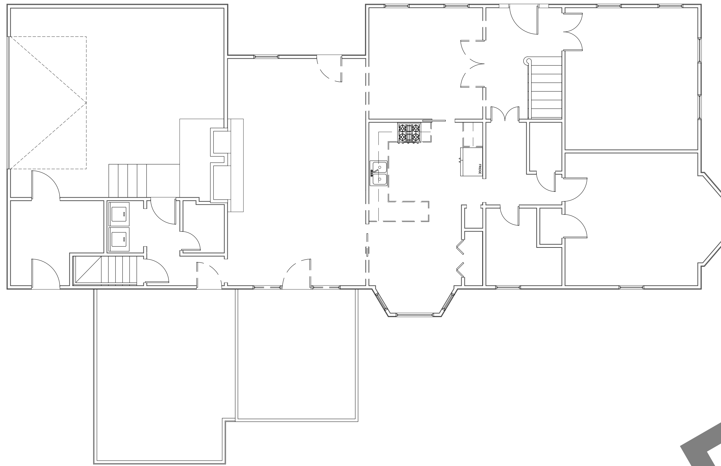
1 AD-101 DEMO / EXISTING SECOND FLOOR PLAN Scale: 3/16 = 1'-0"
