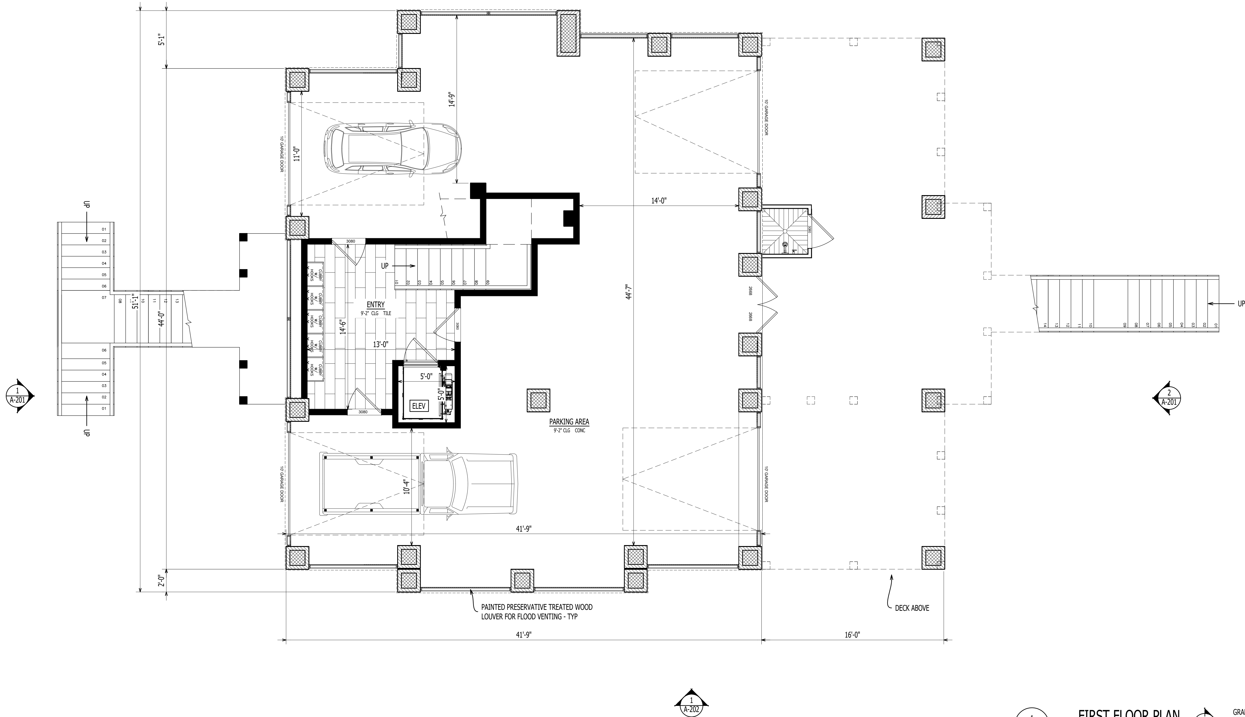
1 FIRST FLOOR PLAN Scale: 1/4" = 1'-0"
