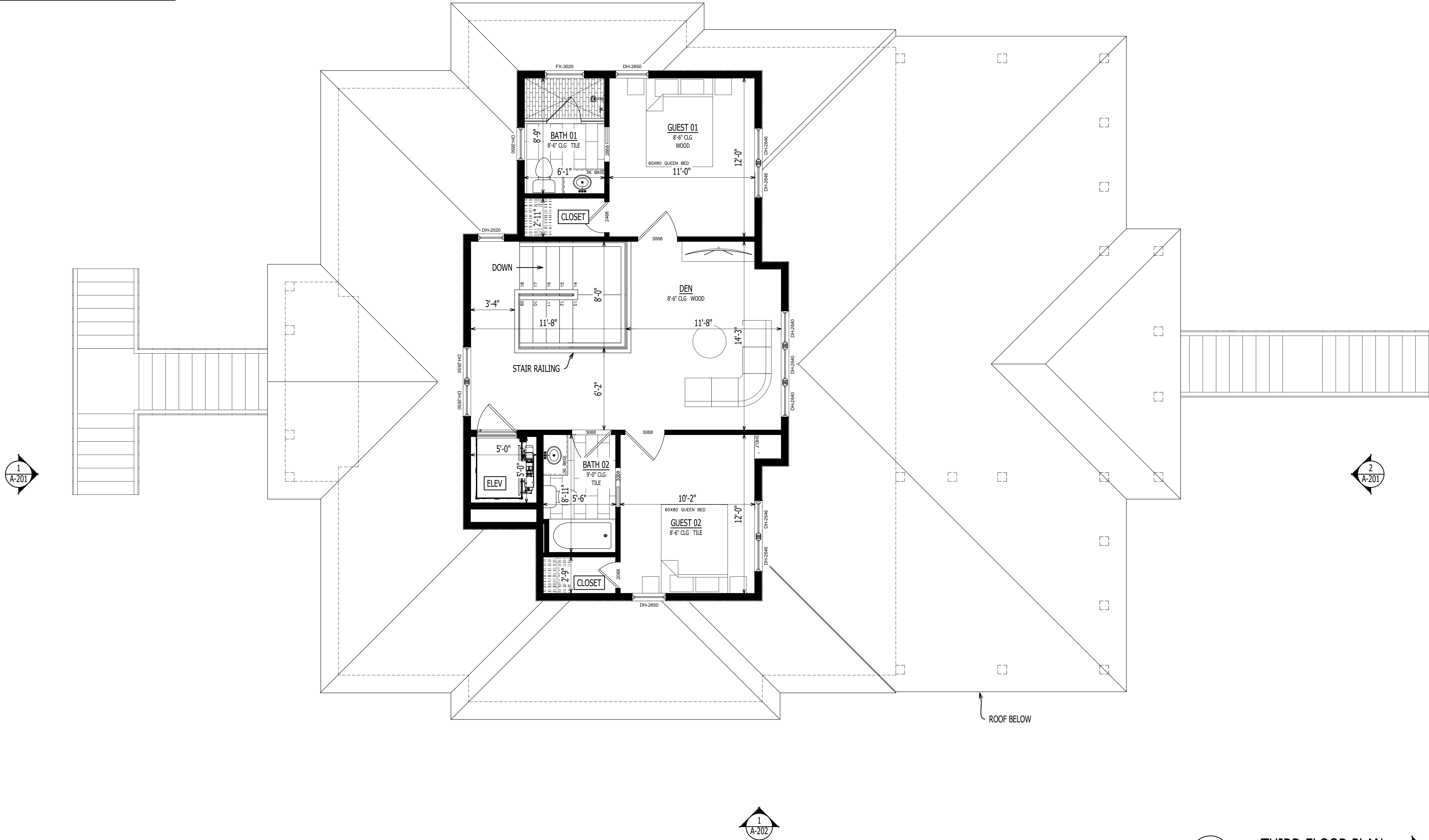
1 A-103 THIRD FLOOR PLAN Scale: 1/4" = 1'-0" 1 2 4 8 GRAPHIC SCALE: 1/4"=1'-0"
